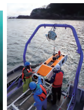
氷海探査用AUV MONACA AUV MONACA for under ice survey
